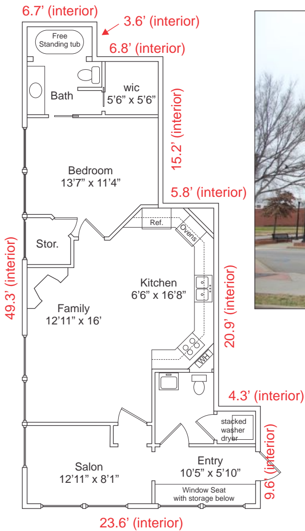
EXAMPLE LAYOUT SHOWING RESIDENCE AND ONE ROOM STYLING SALON WITH WAITING AREA AND RESTROOM
